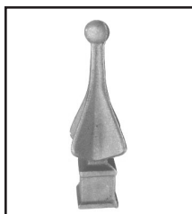
CAST IRON SPEAR 4 1/4" high. Fits 1/2" square tube. 25343 4 1/8" high. Fits 3/4" square tube. 25356 7 7/8" high. Fits 1" square tube. 1 3/4" base.
