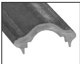
WIDE STEEL HANDRAIL Wide series for 1 1/2" channel. Flat or tube. 20' length. Weight 42.0 lbs.
